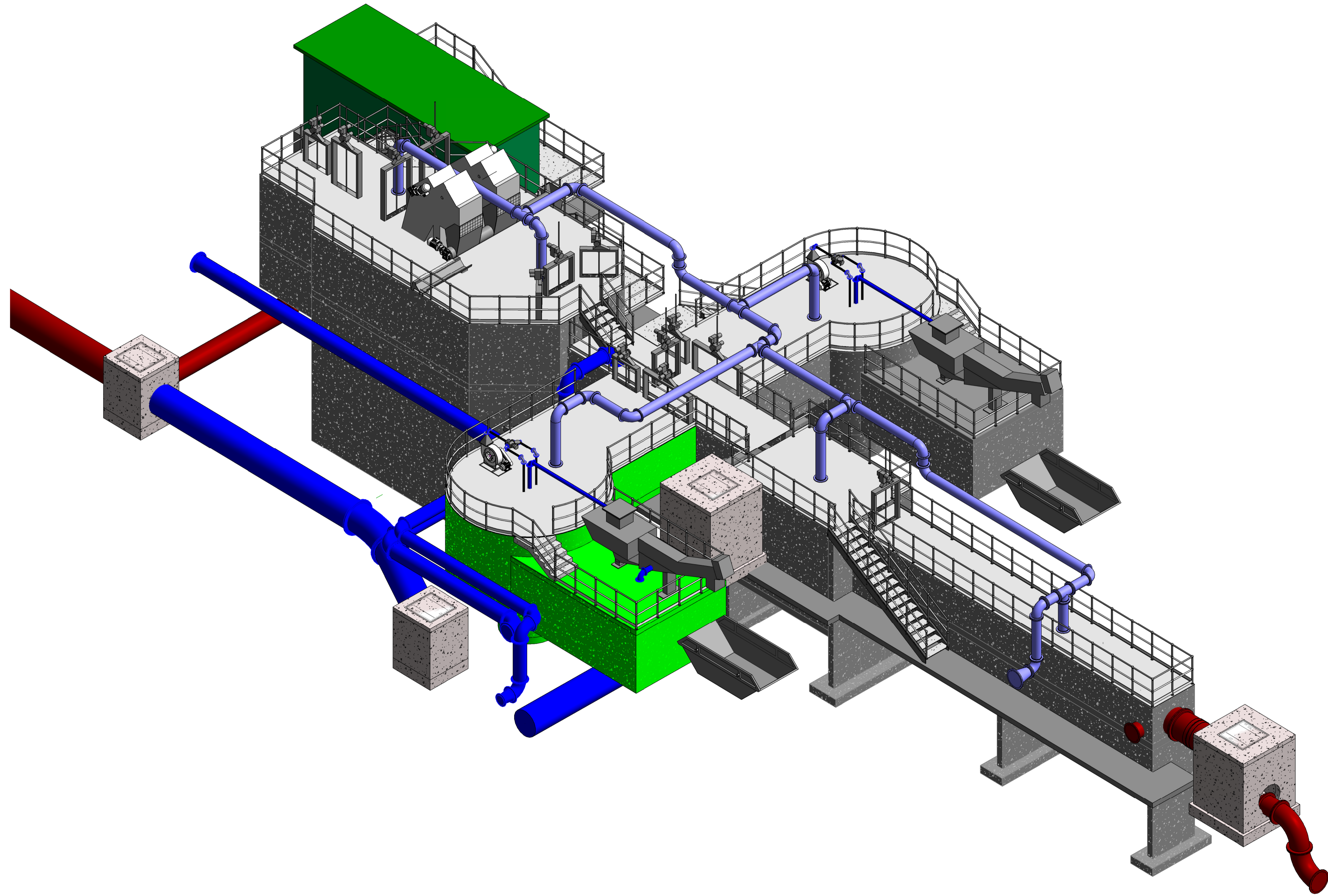
6 3D View of Inlet Works
